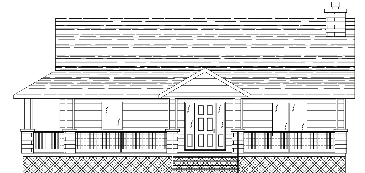
FRONT ELEVATION
